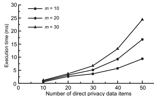
Fig. 6 Time cost of Evolution operation 2.1
