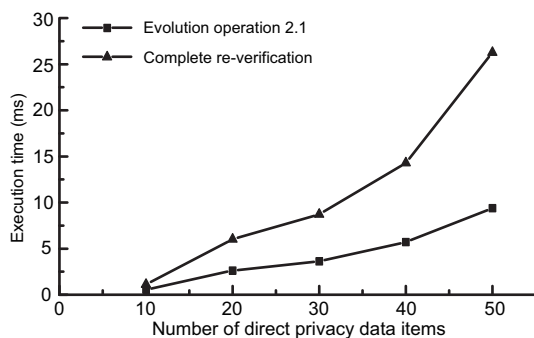
Fig. 7 Time cost by Evolution operation 2.1 and complete re-verification ( m = 10 )
