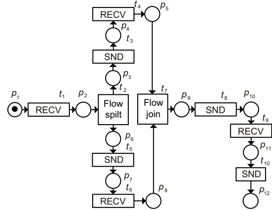
Fig. 5 Control view of the travel agent
