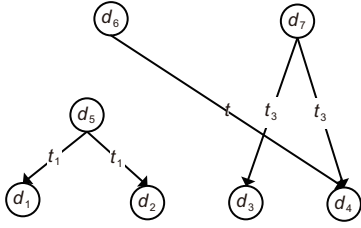
Fig. 2 An updated privacy data item dependency graph
