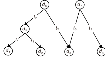
Fig. 1 An example of a privacy data item dependency graph
