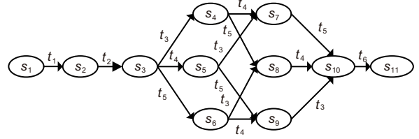
Fig. 4 An example of a coverability graph
