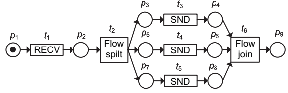
Fig. 3 An example of the control view of a PWF-net
